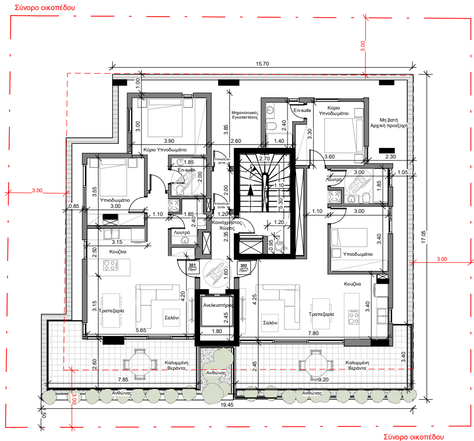
3rd Floor
