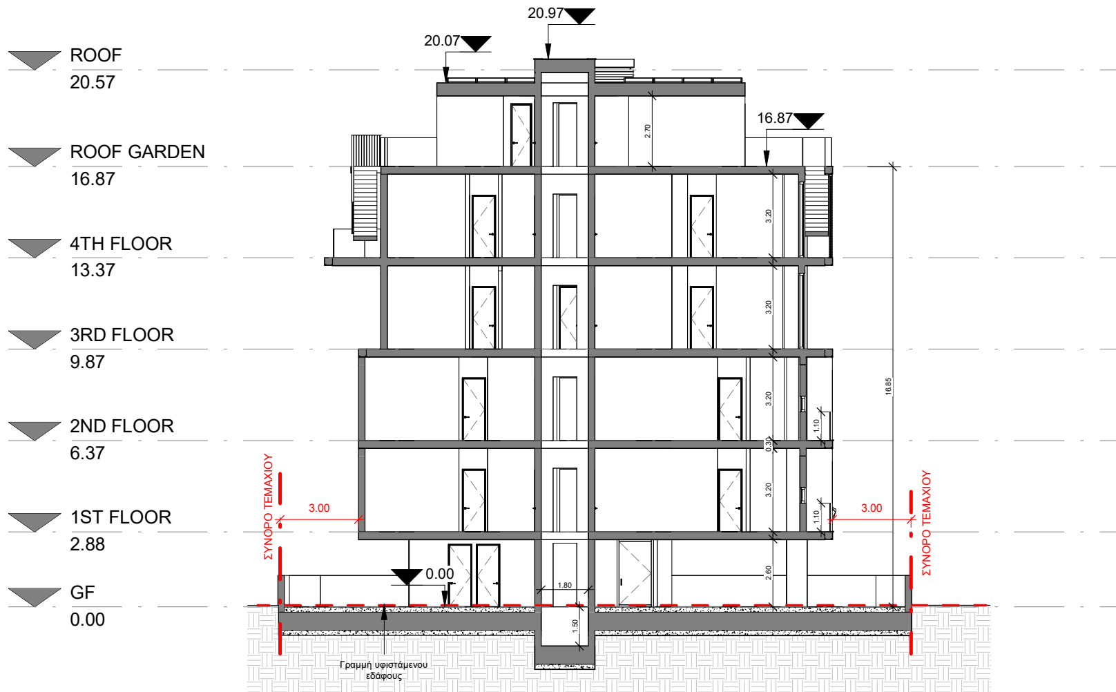
Section B
