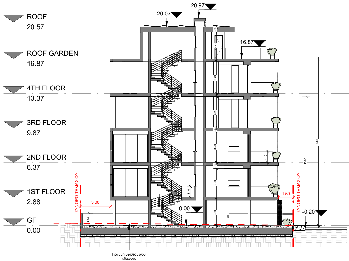
Section A
