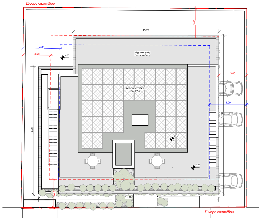
Roof Plan
