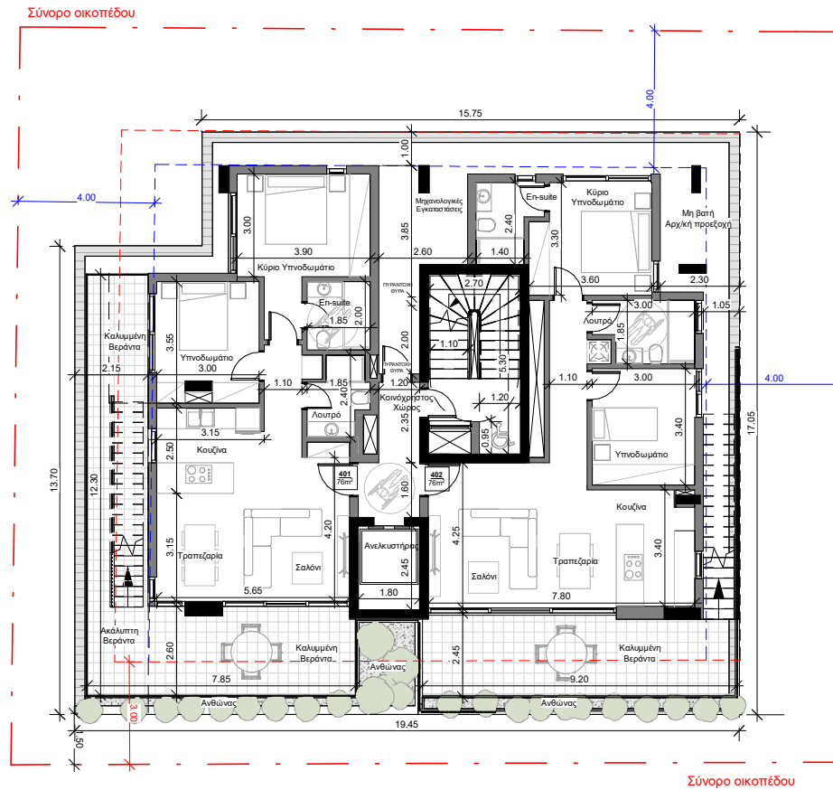
4th Floor
